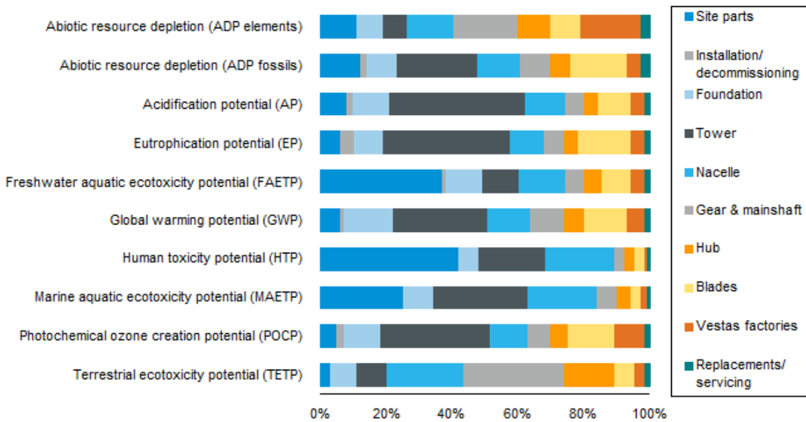
Figure 7: Production and use-phase environmental impacts of V105-3.45 MW
