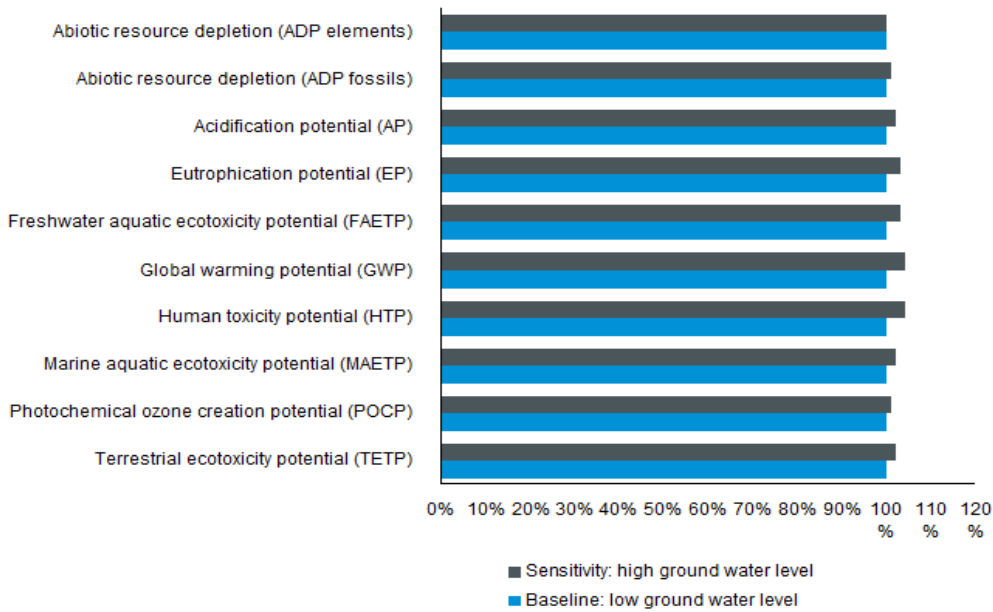
Figure 25: Whole-life impacts for changing from LGWL to a HGWL foundation
