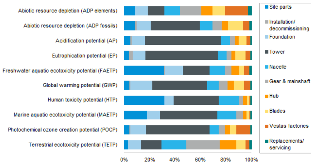
Figure 7: Production and use-phase environmental impacts of V136-3.45 MW
