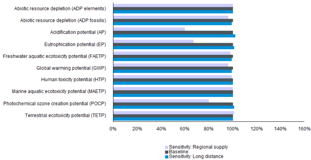
Figure 23: Whole-life sensitivity analysis of increased transport
