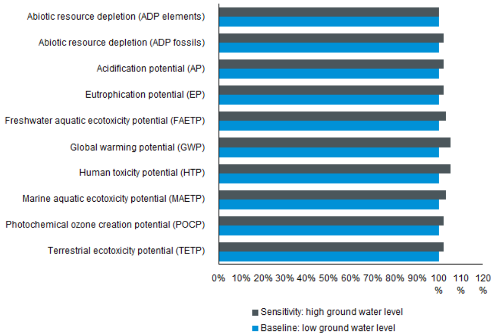
Figure 25: Whole-life impacts for changing from LGWL to a HGWL foundation
